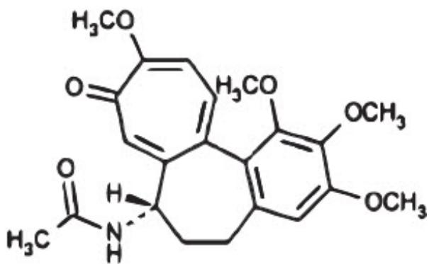
Figure 1: Colchicine Structural Formula
